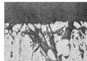
Bending test of a standard hard chrome coating. Poor adhesion, large parts of the coating have come loose.
