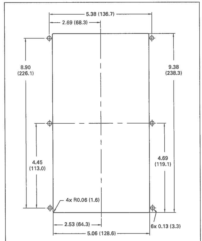
Figure 1. Dimensions of the Cutout Required to Accommodate the Optional Remote Display Panel
