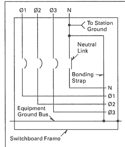
Figure 21.0-1. Neutral Link
