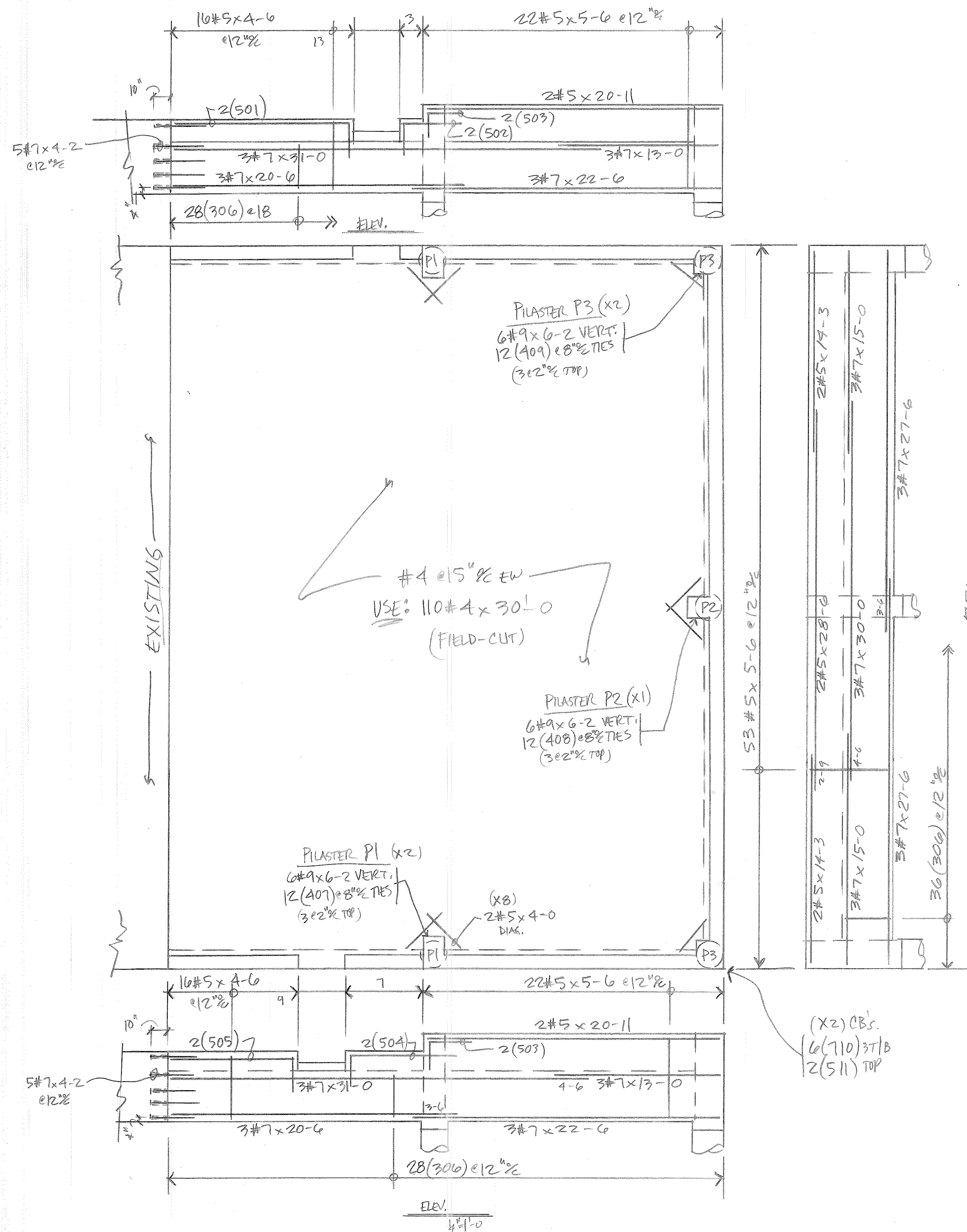
FOUND. PLAN 4"=1'-0"
