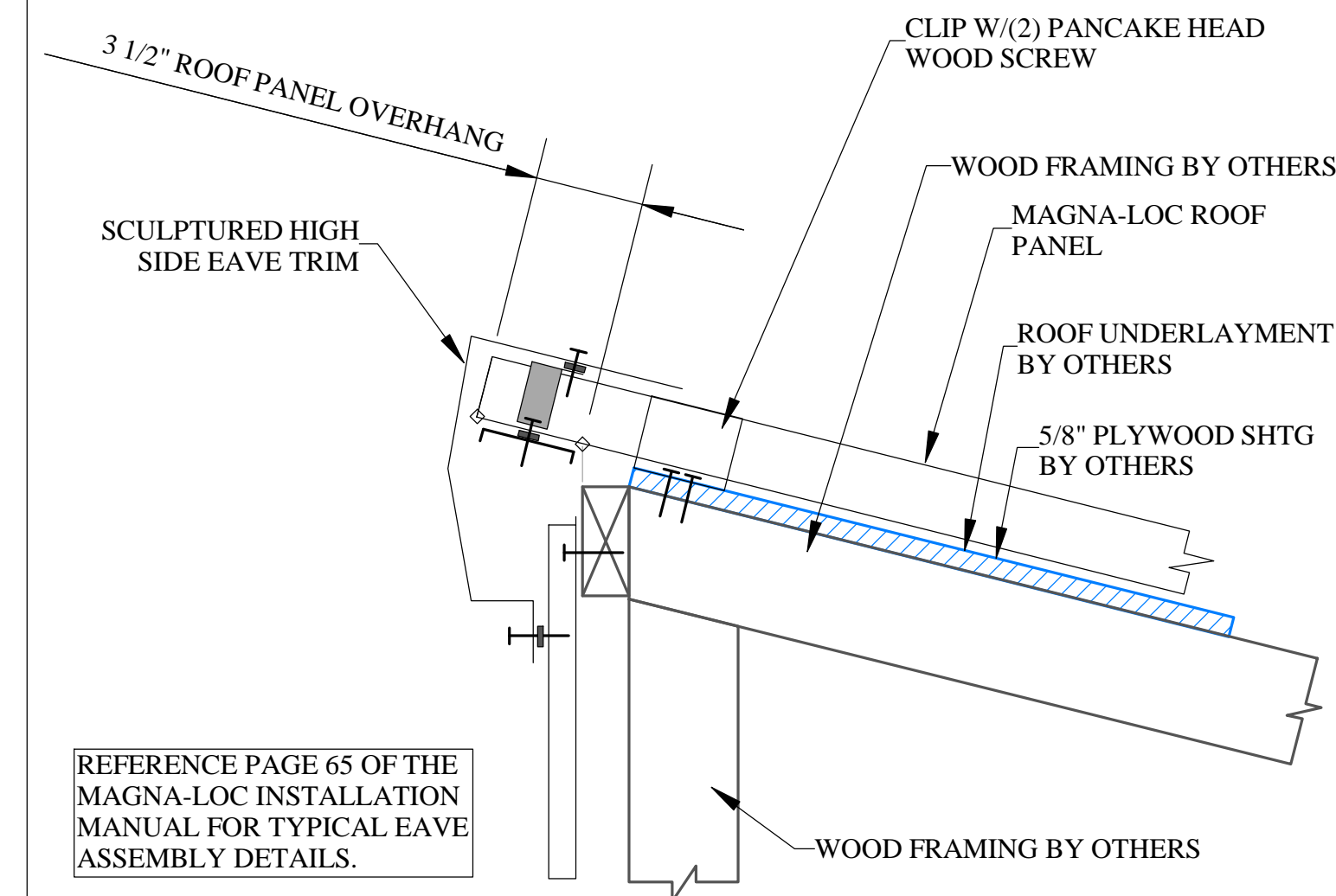
ROOF PANEL PLACEMENT AT HIGH EAVE DETAIL
