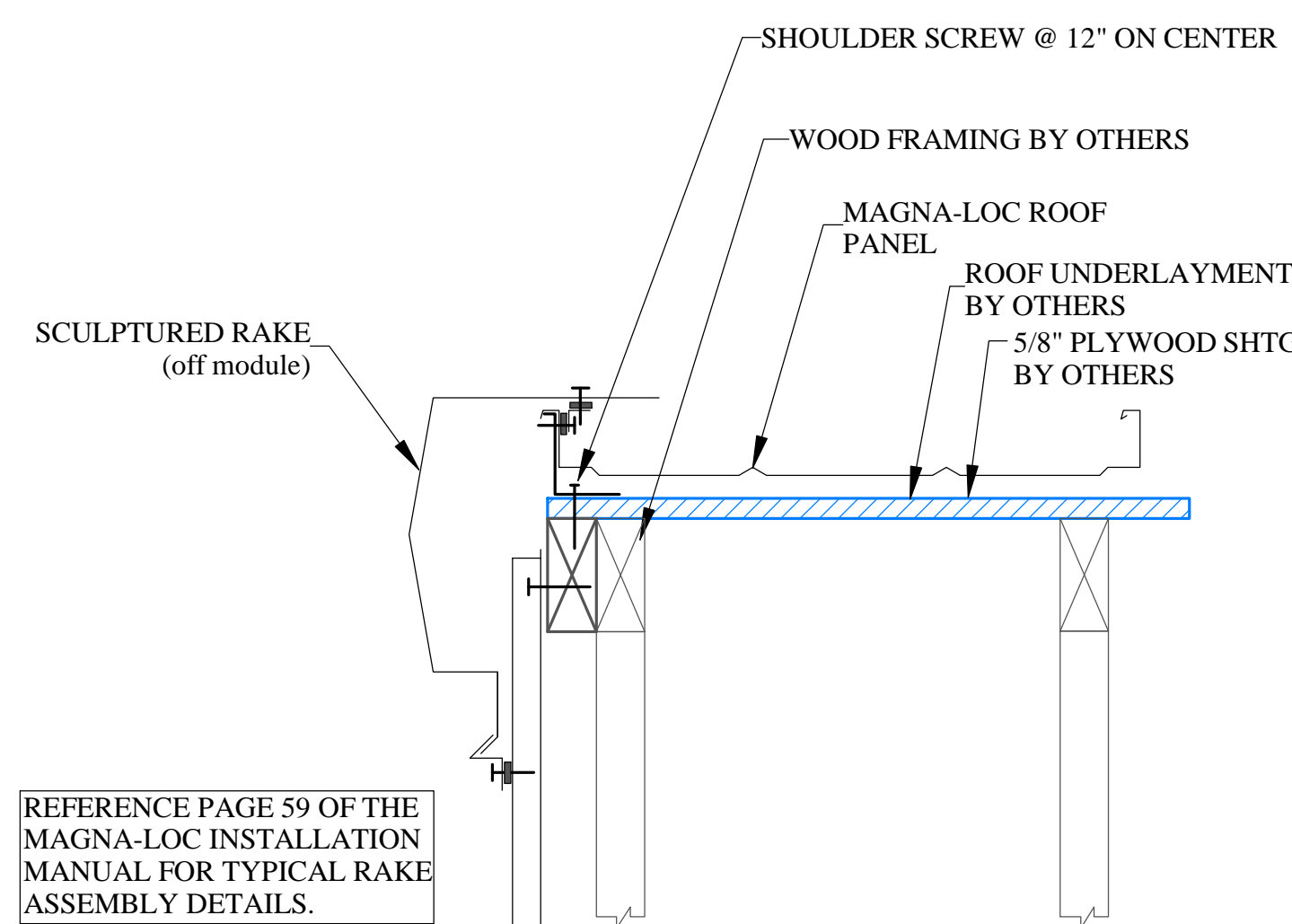
ROOF PANEL PLACEMENT AT RAKE DETAIL
